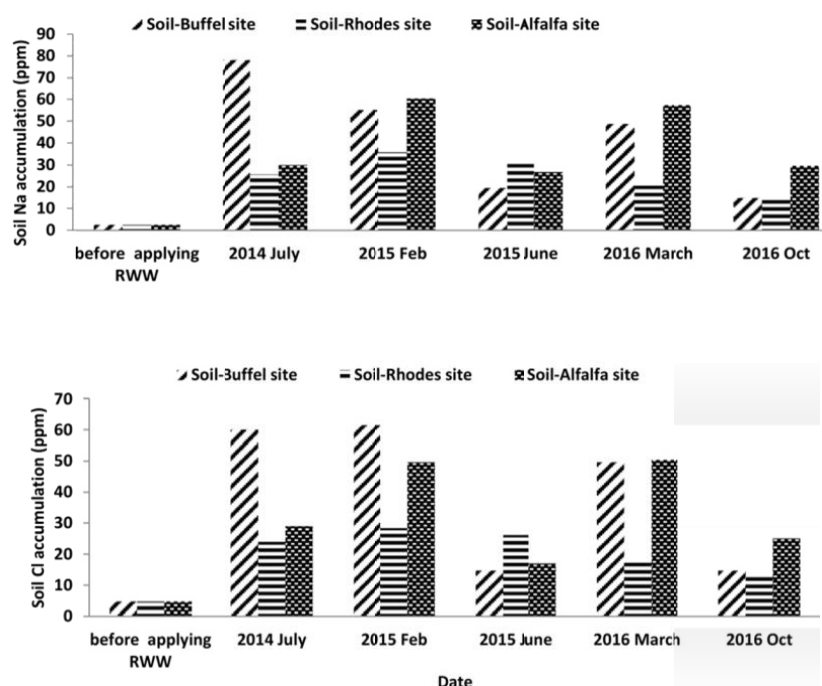
Figure 4. Sodium (Na) and chlorine (Cl) accumulations in the root zone at the studied forage crops sites results of irrigation by Reclaimed wastewater
